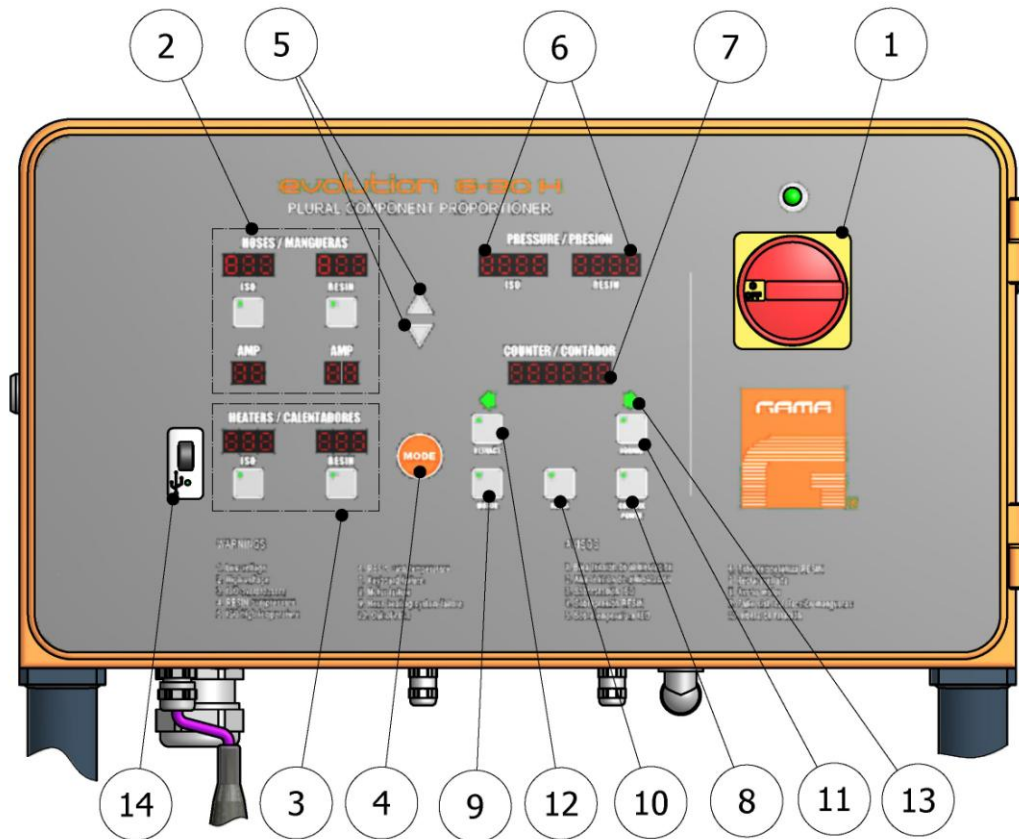
Figure 2. Control Panel
