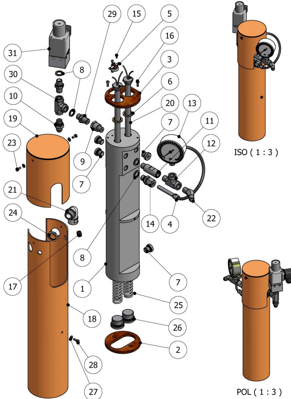
Figure 8. Primary heater
