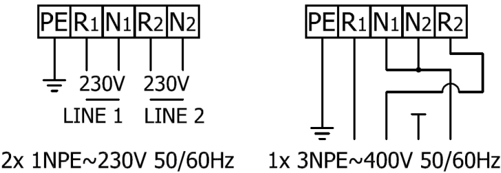
Figure 19. Optional Connections
